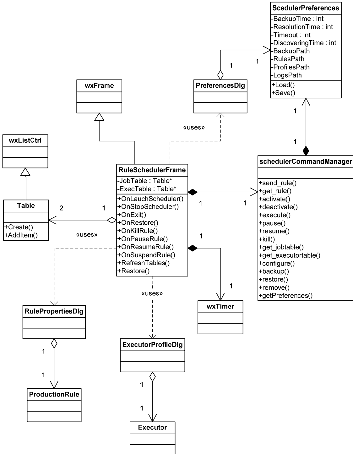
Class diagram of Scheduler GUI
