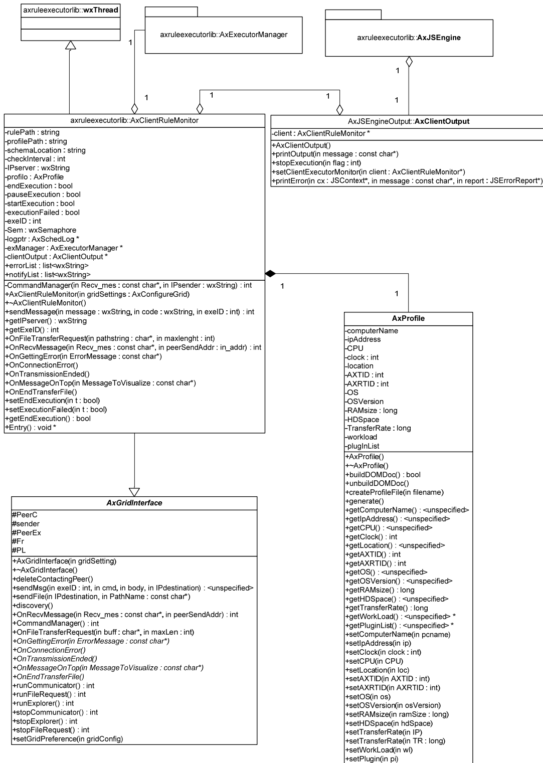
AXCP Grid Node
