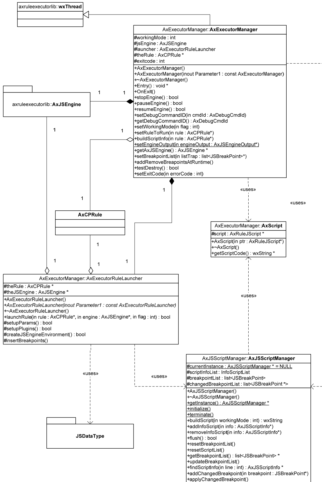
Rule Executor Class Diagram: Executor Manager & Launcher
