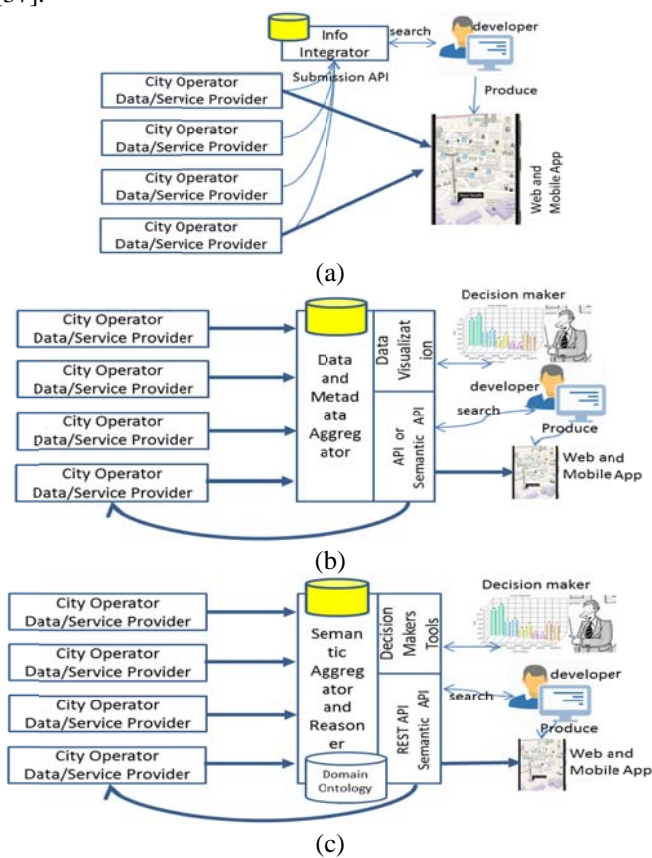
Figure 1: From Data to Services of Smart City Architectures: comparison of different solutions and generations. (description in the text). The thicker lines carry data streams and data services.
